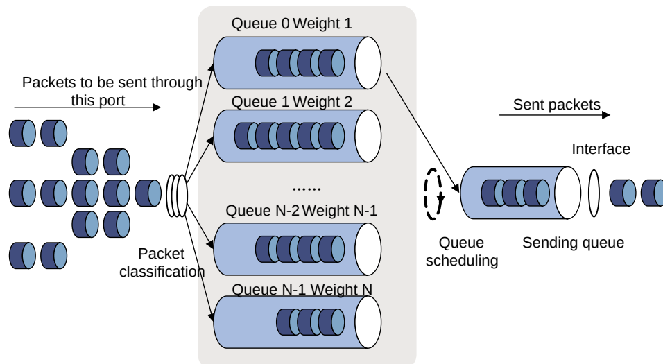
Figure 10 WRR queuing
