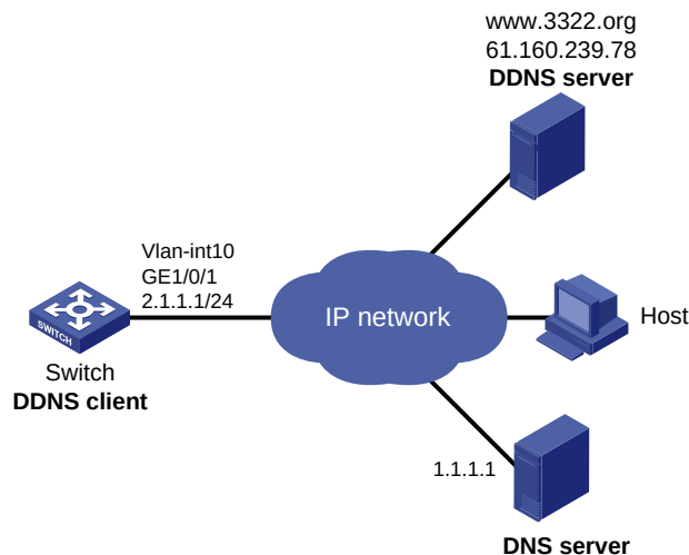
Figure 28 Network diagram
