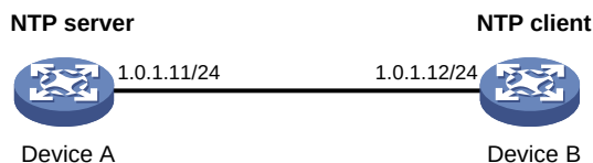
Figure 15 Network diagram
