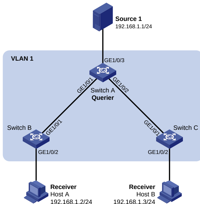
Figure 34 Network diagram
