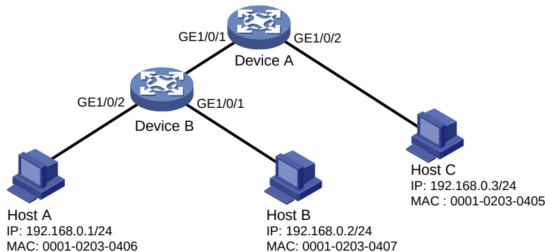
Figure 40 Network diagram
