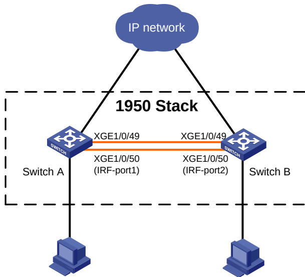
Figure 14 Network diagram
