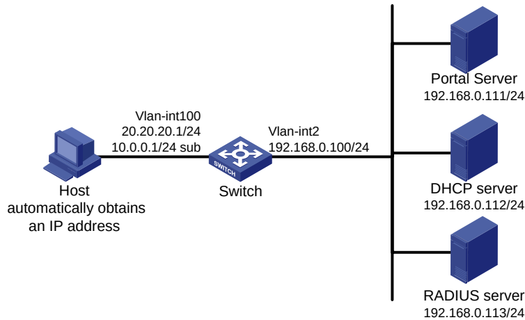
Figure 46 Network diagram
