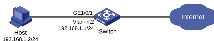
Figure 42 Network diagram
