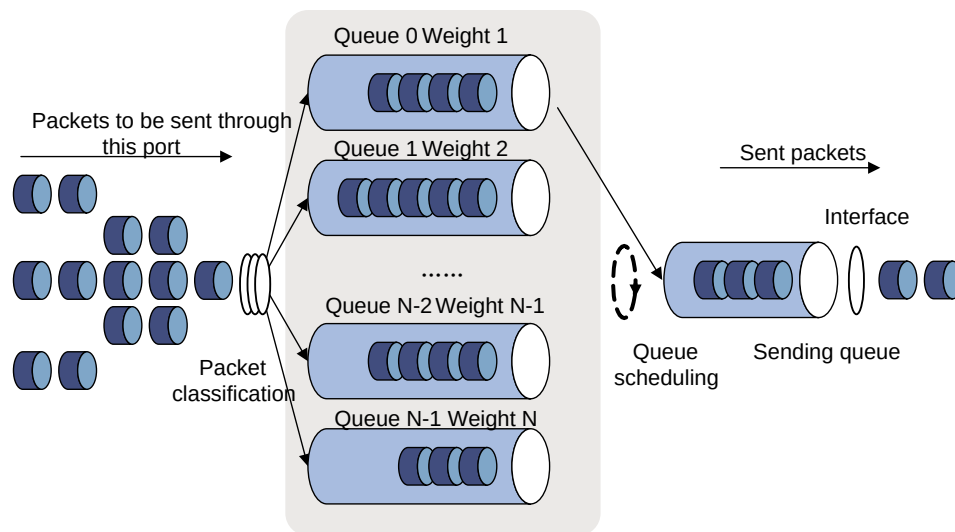
Figure 11 WFQ queuing
