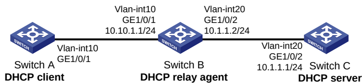
Figure 36 Network diagram
