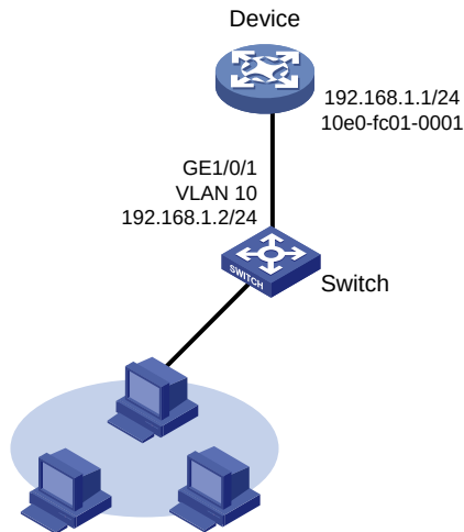
Figure 25 Network diagram
