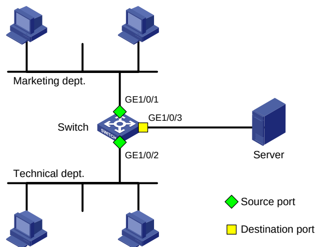
Figure 31 Network diagram
