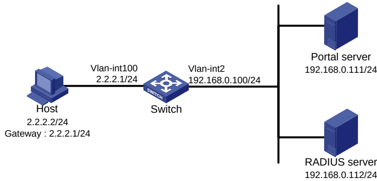
Figure 45 Network diagram
