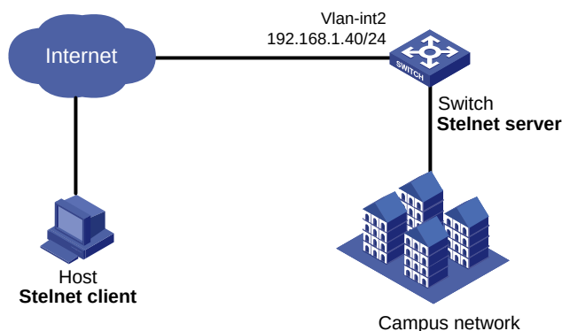
Figure 37 Network diagram
