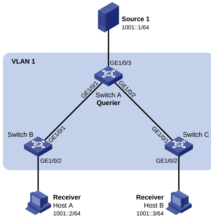
Figure 35 Network diagram
