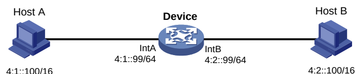
Figure 7 Application environment of common ND proxy
