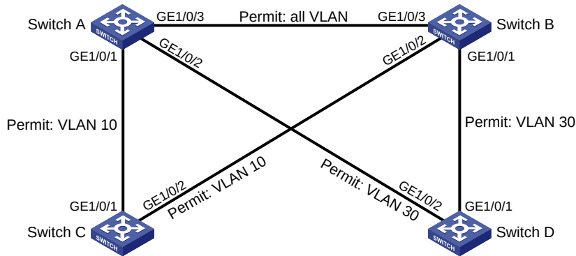
Figure 22 Network diagram
