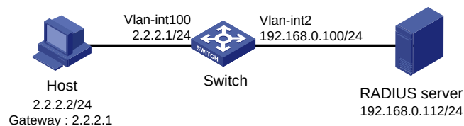
Figure 48 Network diagram
