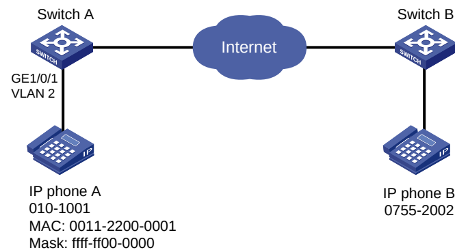
Figure 20 Network diagram
