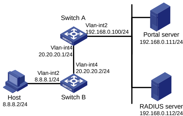
Figure 47 Network diagram
