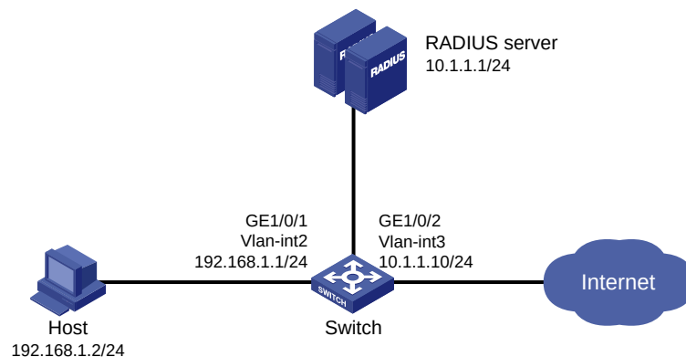
Figure 43 Network diagram
