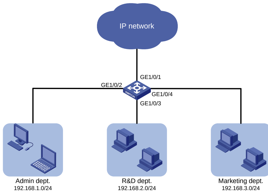
Figure 38 Network diagram
