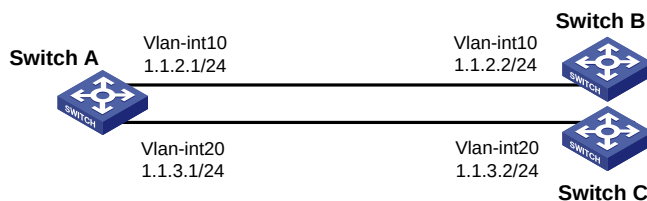
Figure 33 Network diagram
