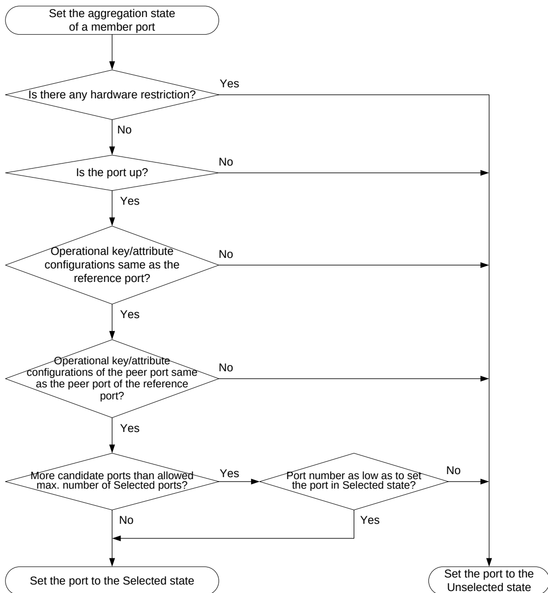
Figure 6 Setting the state of a member port in a dynamic aggregation group
