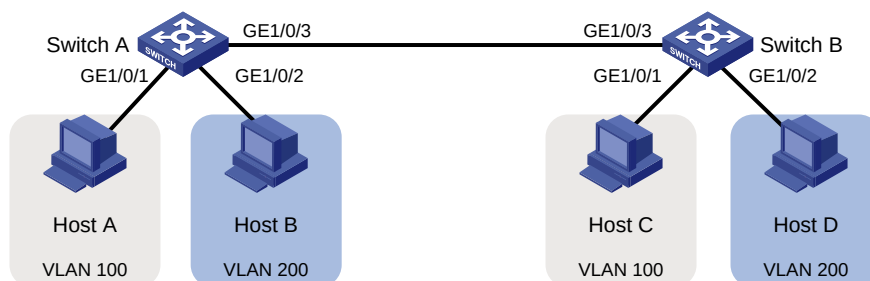
Figure 19 Network diagram
