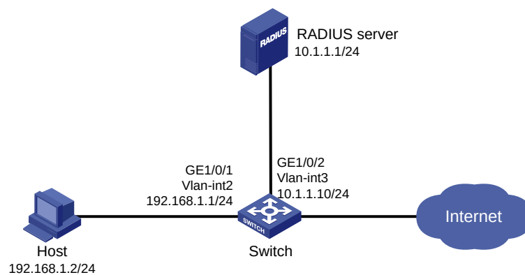
Figure 41 Network diagram
