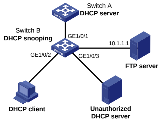
Figure 24 Network diagram
