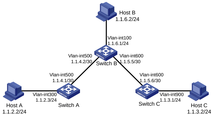
Figure 32 Network diagram
