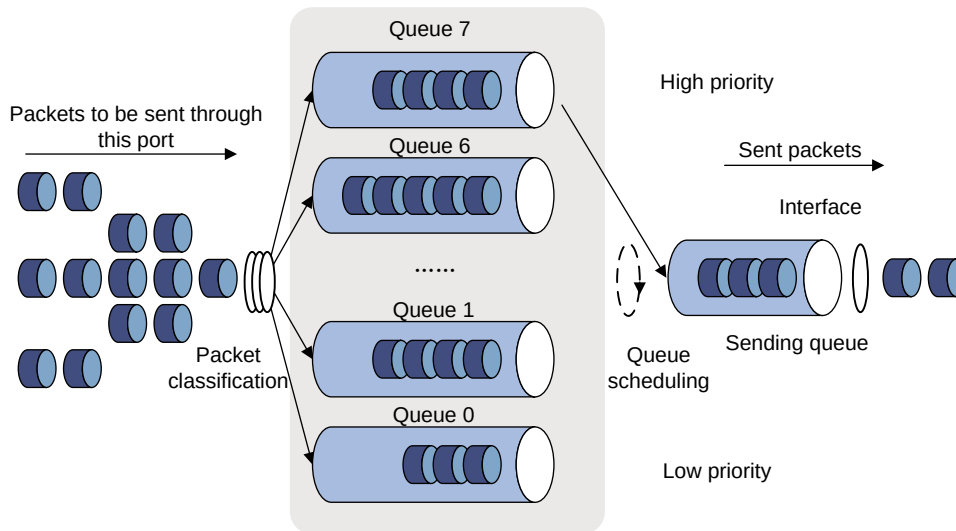
Figure 9 SP queuing
