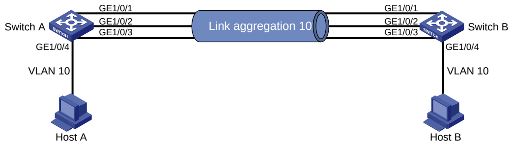
Figure 17 Network diagram
